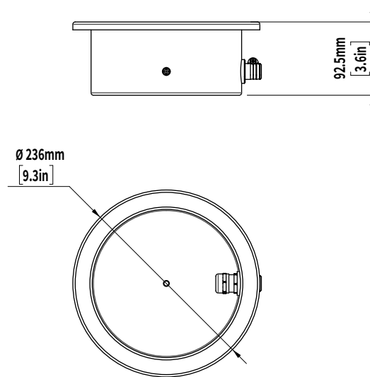
FAL370SP -Stainless Steel Pool Installation
