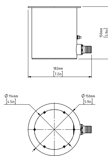
Installation housing AXMSP *fits 1m (3,3') cable Stainless steel pool installation trim
