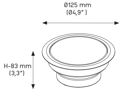
Trim (TM)
