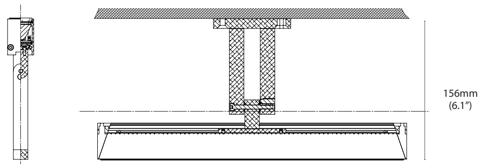
Extended adjustable bracket (AE)
